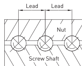
Fig. 2.16 Preload from ball size
