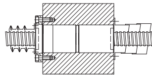
Fig. 2.4 Telescopic or bellows shaft protection
