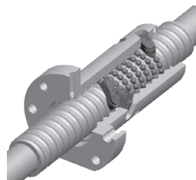
Fig. 1.6 Internal recirculation type nut with return caps (RSI type)
