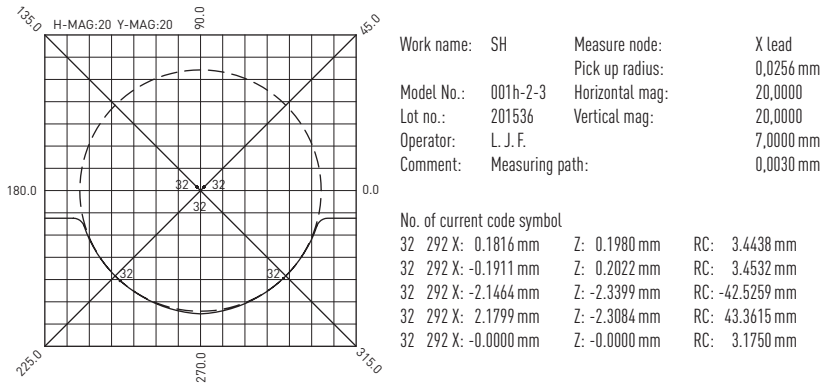
Fig. 1.3 Ball arch profile testing at HIWIN
