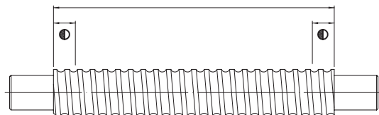
Fig. 2.6 Area of surface hardening on a ballscrew shaft
