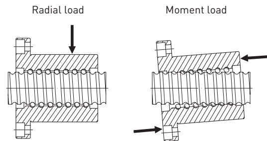
Fig. 2.1 Uneven load distribution , caused by insufficient alignment of support bearing and ballscrew nut, incorrect configuration of mounting surface, incorrect angle or error in aligning the nut flange
