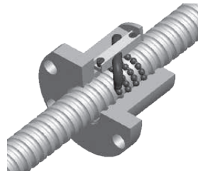
Fig. 1.5 External recirculation type nut with return tubes
