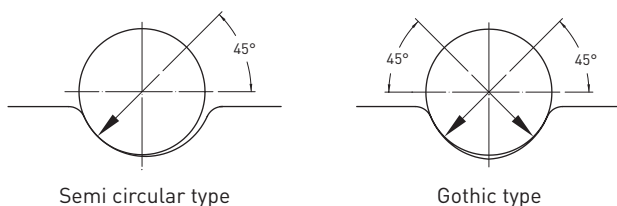
Fig. 1.2 Typical types of contact in ballscrews (semi circular type, gothic type)
