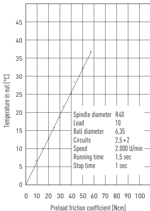
Fig. 2.25 Relationship between temperature increase in the ballscrew and idle torque
