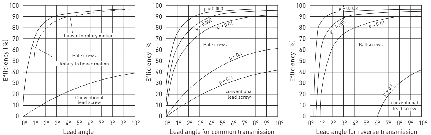
Fig. 1.1 Mechanical efficiency of threaded shafts
