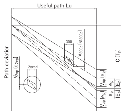
Fig. 2.11 DIN measurement curve of lead of ballscrews
