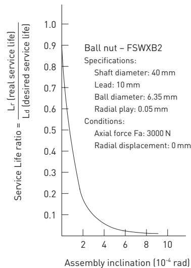
Fig. 2.2 Impacts on life expectancy of radial load caused by insufficient alignment
