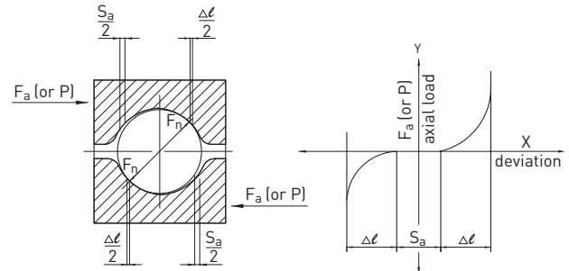
Fig. 2.14 Gothic arch profile and preload
