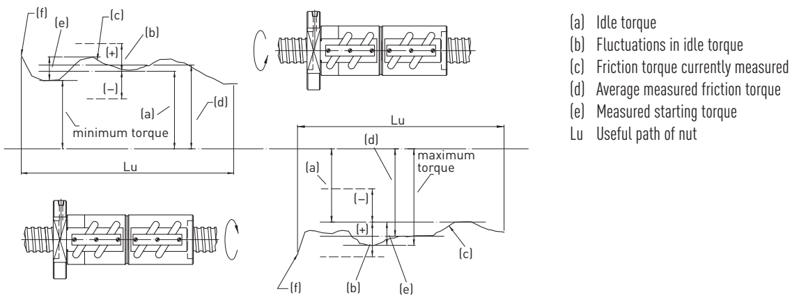
Fig. 2.18 Nomenclature for measuring idle torques
