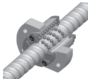
Fig. 1.7 Endcap recirculation type nut with recirculation system (FSC type)
