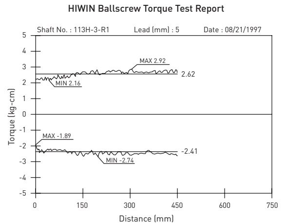
Fig. 1.4 Preload testing at HIWIN
