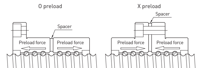
Fig. 2.15 Preload from spacer
