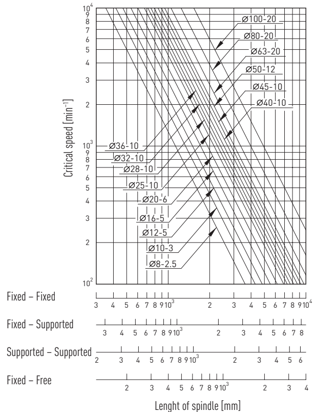
Fig. 2.21 Critical speed for different diameters and lengths of threaded shafts
